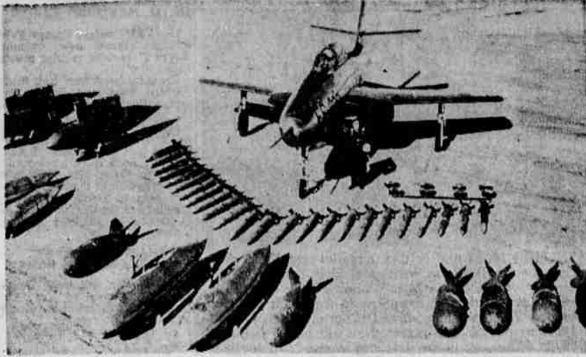
FUTURE FIGHTER UNVEILED —A future fighter-bomber, Republic F-84F swept-wing Thunderjet, sister ship of the F-84E now in use in Korea, is unveiled at El Segundo, Calif. As proof of its versatility, the plane is shown with the five-inch rockets, four 1000-pound bombs, napalm tanks and 230-gallon fuel tanks it can be fitted to carry.
