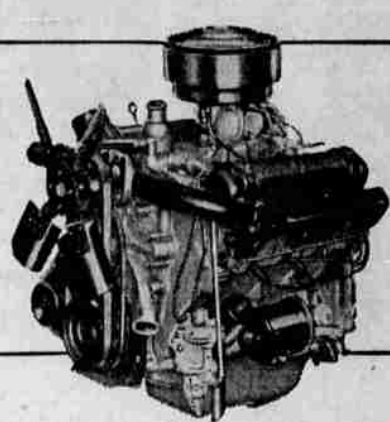
155-h.p. CARGO KING V-8: New LOW-FRICTION design, 317 cu. in. Standard in Series F-8.
