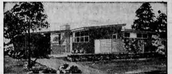
National Plan Service Design LD-212 is a design developed by the University of Illinois Small Homes Council as part of a research project sponsored by the lumber Dealers Research Council.
