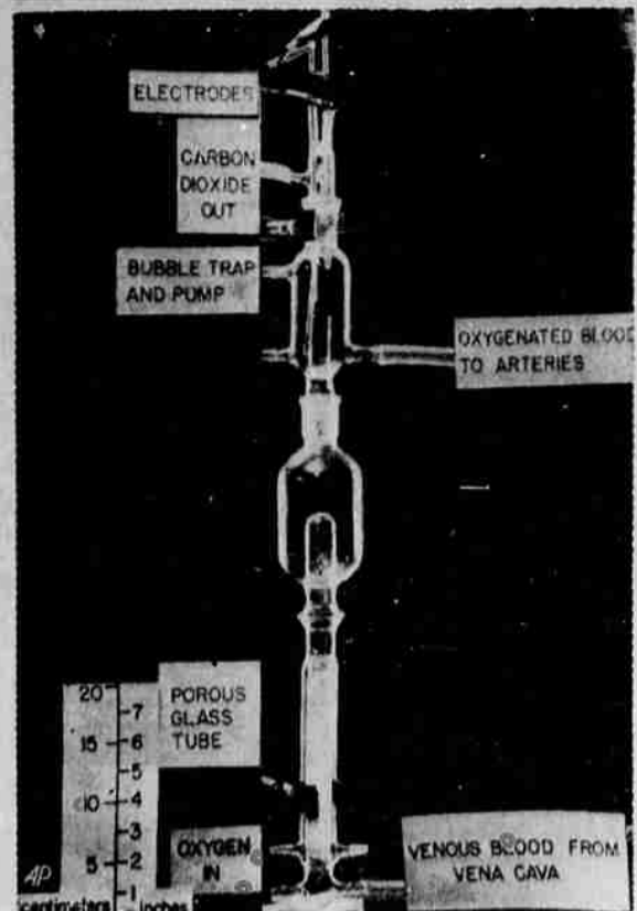
ARTIFICIAL HEART-LUNG —This artificial heart-lung, simple enough to be built in any laboratory, has been developed by scientists at Fels Institute, Yellow Springs, O. Made of glass, the instrument has no moving parts. Valves control alternating pressure and suction duplicating the heart's "pumping". Among its uses is an emergency means of by-passing the heart and lungs while surgeons repair those delicate organs. (AP Wirephoto)
