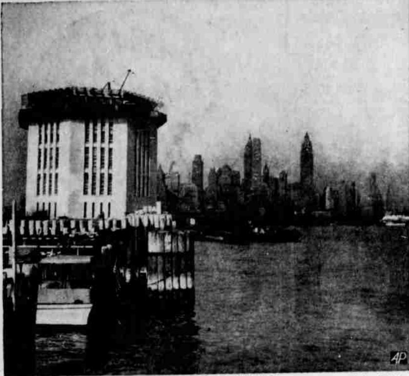
VENTILATOR FOR 9,117-FOOT TUNNEL —One of four ventilation buildings for New York's Brooklyn-Battery tunnel to open soon stands between Governors Island (foreground) and Manhattan skyline. $80,000,000, 9,117-foot tunnel links lower Manhattan with Brooklyn.
