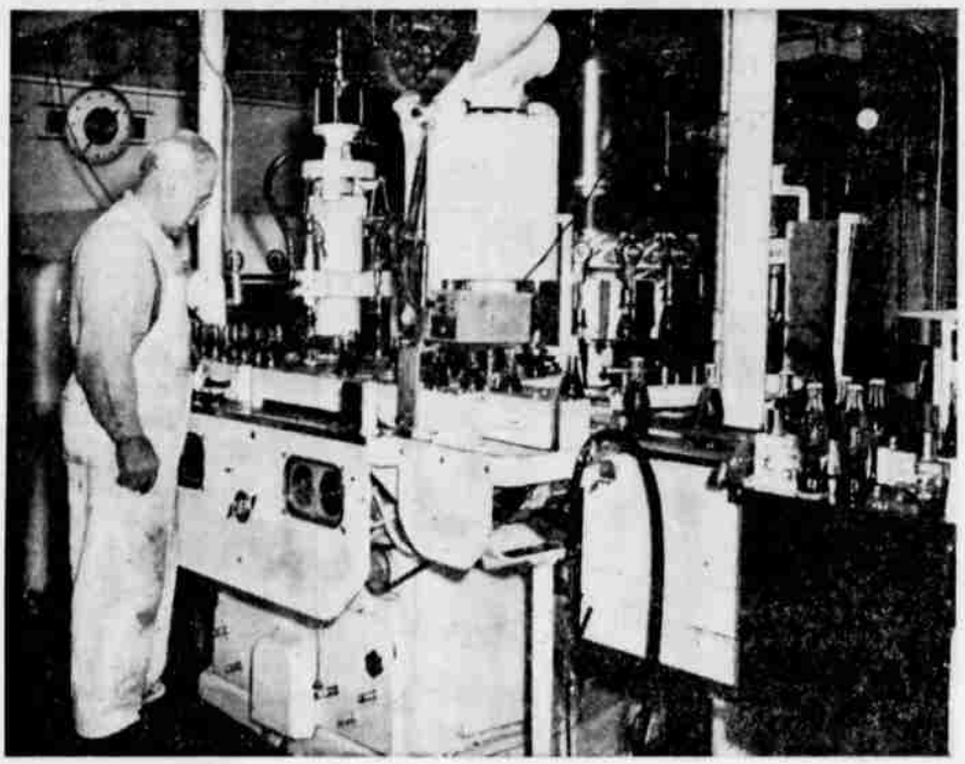
ERNEST UNRATH , president of the Roseburg Coca-Cola Bottling company, is shown as he presides over the filling and carbonating machine in his immaculate plant. The unit fills the bottles with Coca-Cola syrup and carbonated water which has passed through a de-chlorination and filtering process. It caps them, mixes the contents by spinning the bottles and passes them along the line to the accumulating table.—(Picture by Paul Jenkins.)
