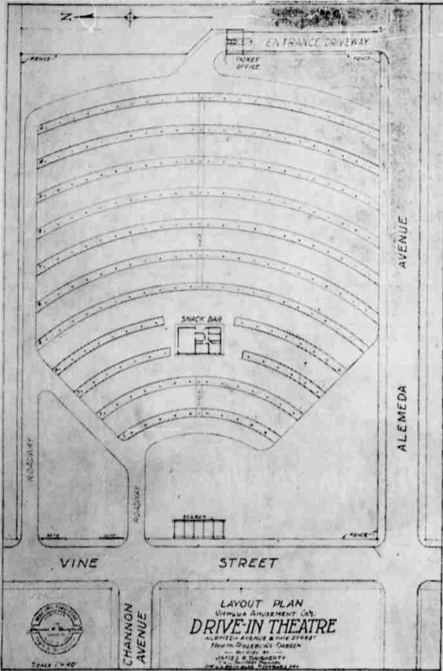
DRIVE-IN THEATER PLAN SHOWN —Above is the designer's sketch plan of the new drive-in theater to be located in North Roseburg. The plan was prepared for the Umpqua Amusement company by James R. Daugherty, local engineer.
