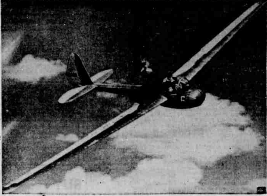
GLIDER AIDED BY OUTBOARD MOTOR —This sailplane in flight over the Arlington State college airport at Grand Prairie, Tex., uses an auxiliary motor, visible back of cockpit, to get into the air instead of the conventional tow rope. Motor folds forward into the plane's body after ship gains enough altitude to soar. Ted Nelson of Oakland, Calif., builder of the plane is at controls. (AP Wirephoto)
