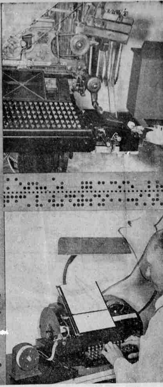
TELETYPESETTER INSTALLED BY NEWS-REVIEW —Pictures above show major parts of the Teletypewriter unit now in operation in the News-Review's mechanical department. Photo at lower right shows the perforator where an operator works at a standard typewriter keyboard to which is added various keys conforming to linotype operations. The perforator punches combinations of holes in tape. Large photo shows transmitter and keyboard attached to a linotype. Tape fed into the transmitter sets up electric impulses which are transformed into mechanical action on the keyboard, producing automatic operation of the line-caster. Photo upper right is a close-up of the transmitter and keyboard. The Teletypewriter will operate a linotype at about twice the speed normally obtained in manual operation. The News-Review's machine is to be used in auxiliary capacity and will not replace any present personnel. (Pictures by Paul Jenkins.)
