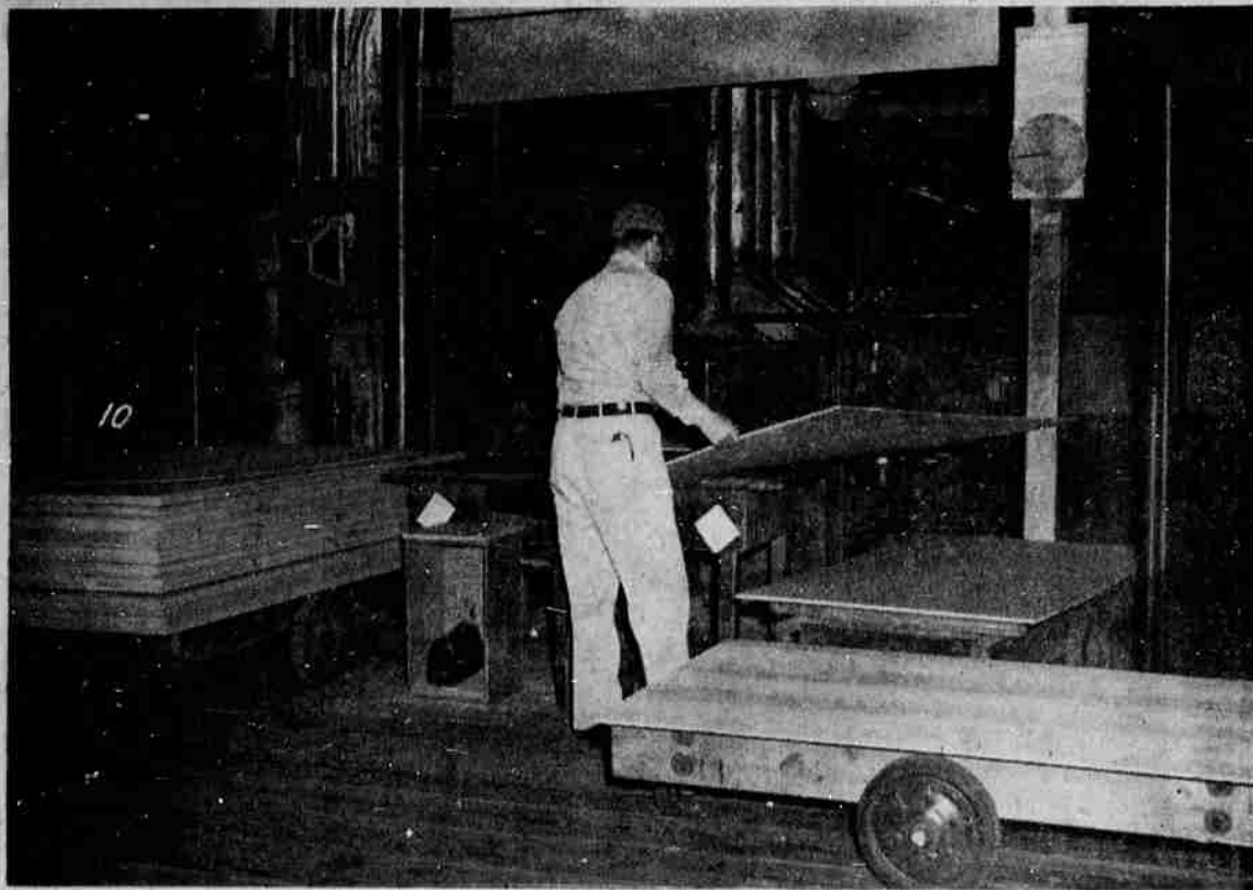
FINAL STEPS —With trimming and sanding, the plyboards are ready to be shipped from the plant. These pictures show: (9) Operation of panel trim saws, and (10) sanding machines. These scenes are typical of the operations of the Associated Plywood Mills, Inc., at its plants in Eugene and Willamina.
