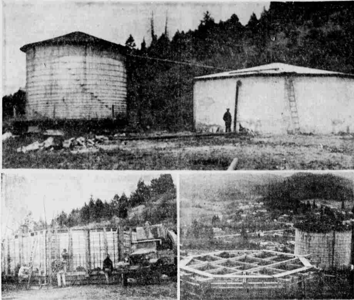
WATER RESERVOIR COMPLETED —A new, 100,000-gallon water reservoir was recently completed at Canyonville. Octagonal in shape, it was designed by James R. Daugherty, Roseburg engineer, as the first of two such reservoirs. Top picture shows the completed reservoir at right, and old 50,000-gallon wood stave reservoir which will be used until the second new tank is constructed. Most walls of the new reservoir are eight-inch thick concrete, heavily reinforced. They were poured monolithic by using special plywood panel forms suspended from a trussed framework. Eighty cubic yards of concrete were used and 13,000 lineal feet of 8-inch reinforcing steel. The concrete tank was designed originally for a steel-framed aluminum roof. The work was done by force account under supervision of Merle Fuller, foreman, when no bids were received by the city. Lower pictures show construction scenes. (Upper picture by Paul Jenkins, lower pictures by James R. Daugherty.)
