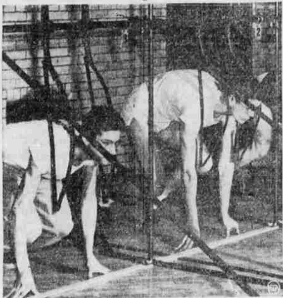
Temple track coach Ben Ogden devised this contraption for eliminating false starts. Product of many years work, the gate has an automatic phototiming device to go along with it.
