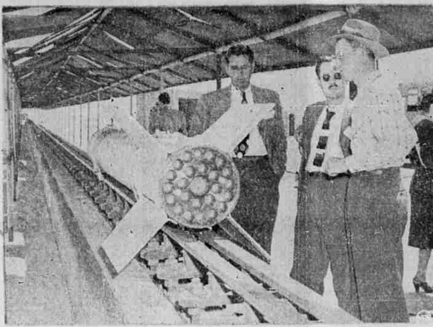
"Tiny Tim" rocket rests on 1500-foot launching rail as Ray Nelson (right) explains its operation to newsmen at dedication of Mehl's laboratory at Insokern, Calif. Part of the Naval Ordnance Test Station here, the new laboratory is an extensive research facility for propulsion systems for rockets and missiles. The launch is the all-weather, fire control and guidance testing room. The launch is 1500 feet long.
