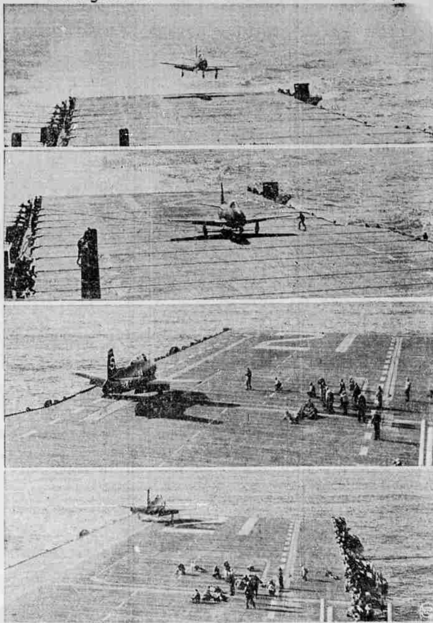
Operational jet propelled aircraft were landed and flown off a carrier for the first time March 10 when the Navy's newest and fastest plane, the North American FJ-1 "Fury" successfully completed its first trials, aboard the USS Essex off California coast. This dramatic photo sequence shows initial landing and takeoff, described by high officials as "marking the turn in naval aviation." Top photo shows Comdr. E. P. Aund, Houston, Tex., coming over the stern of the Essex and in second photo plane handlers rush out to disengage tail hook after a perfect landing, having caught the No. 1 wire. Note short length of deck used in bringing plane aboard. Landing speed was 105 knots. Third photo in series shows Lt. Comdr. R. M. Elder, Portland, Ore., ready on catapult for first flight off the ship, jet engine turning up full power. A moment later (bottom photo), plane has reached 130 knots speed and leaves deck after 95-foot run on catapult.
