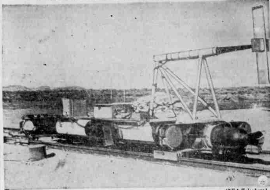
Rocket-powered sleds such as this, streaking along a set of railroad tracks in the desert near Murco, Calif., have attained speeds in excess of 1000 m. p. h., according to Air Force announcement. Experiments were made to determine feasibility of outdoor wind tunnels in which the object being tested would move instead of the surrounding air.
