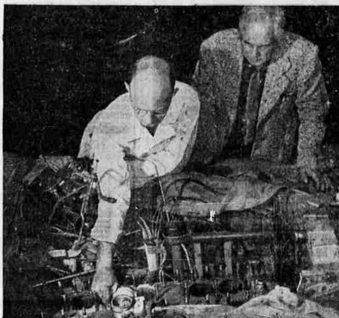
Professor R. L. Daugherty, of Caltech, and associate, examine one of the engines. All engines were still in top condition, though the distance traveled was equal to 3 years normal driving without an oil change!
