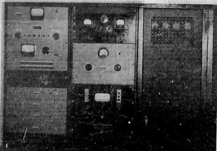
KRNR TRANSMISSION PANEL —Behind the panels pictured above are the glowing tubes and the various pieces of equipment which toss the radio station's signals into the ether. The compact and efficient panel was designed and constructed by Henry (Bud) Chandler, KRNR engineer. This equipment will be seen by persons attending KRNR's Open House to be held from 4 to 7 p. m. Saturday, to which the general public is invited to inspect the station's new home in the Kohlhaugen building.
