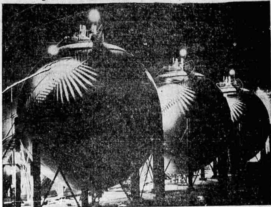
Reflecting the highlights and shadows of night war production, these Hortonaphere storage tanks, part of the new $20,000,000 Defense Plant Corporation refinery operated by Standard of California near San Francisco, hold huge quantities of 100 octane gas destined for Saipan-based B-29 Tokyo raiders and other Pacific aerial operations. The refinery is one of world's largest high octane producers with capacity of several thousands of barrels daily.
