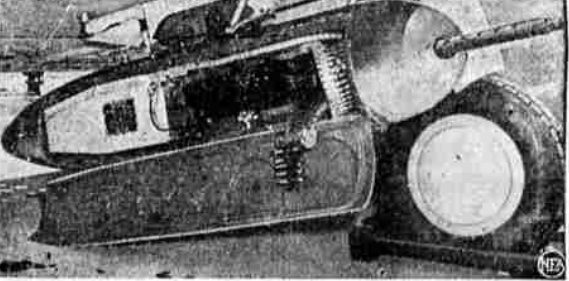
Here is the first picture of the Navy's new "package machine gun," with torpedo-shaped containers opened to show mechanism. Hung under each wing of plane like bombs, a pair of these "packages" contains four machine guns and ammunition, and doubles the firepower of planes mounting four fixed-position guns. Emergency jettisoning of package by usual bomb-release lightens plane's load by 600 pounds.
