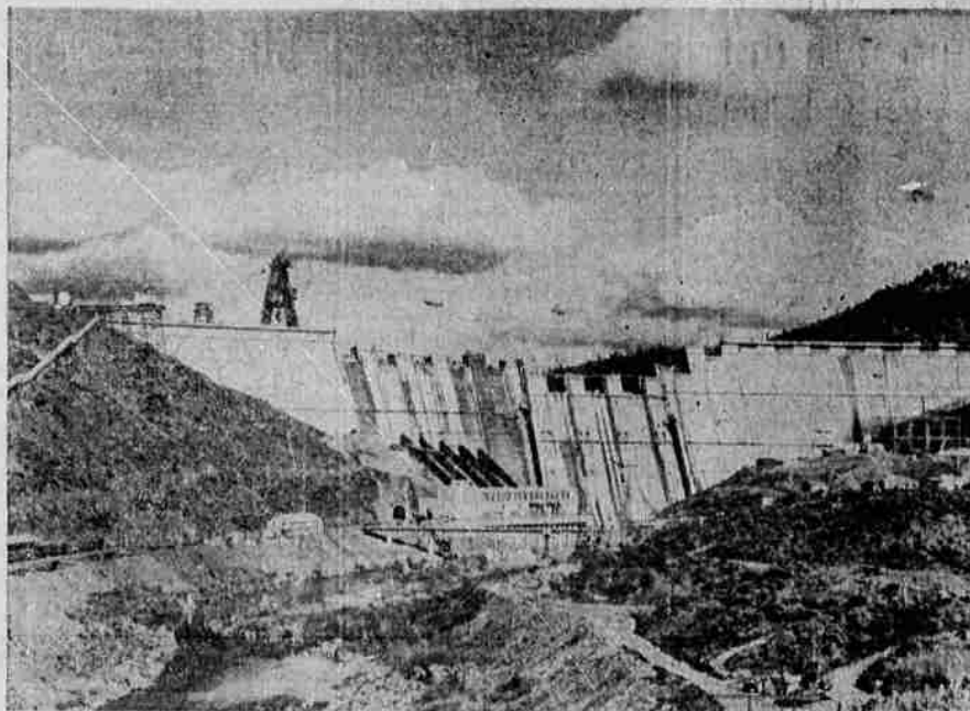
California's giant Shasta Dam is nearly finished with concrete placement scheduled for completion early in July. Shasta Lake already contains 15,000 acre feet of water awaiting the completion of control gates to begin its plunge down the 15-foot spillway to the 75,000-kilowatt generating units in Shasta's power plant. (NEA Telephoto)
