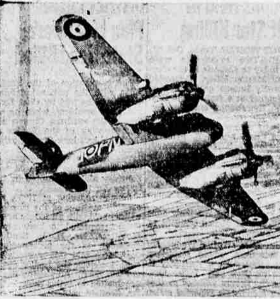
British claim this Beau Fictler is the most powerful air attacker ever built. Weighing 21,000 pounds loaded, the all-metal monster has an admitted speed of 330 miles an hour, range of 1,800 miles and carries four cannon and six machine guns.
