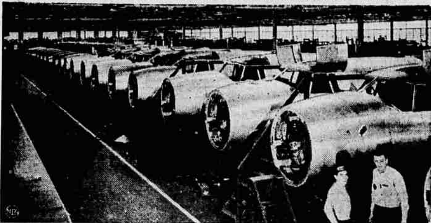
Bodies of Martin B-26 medium bombers stretch out in long row on assembly line awaiting wings and engines in Baltimore plant of Glenn L. Martin, which is producing them in droves for U. S. Army.
