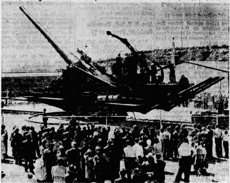
Focal point of attention during Army Day activities at Ft. McArthur, Cal., was this huge 14-inch railway gun mounted and ready to speak in coastal defense.
