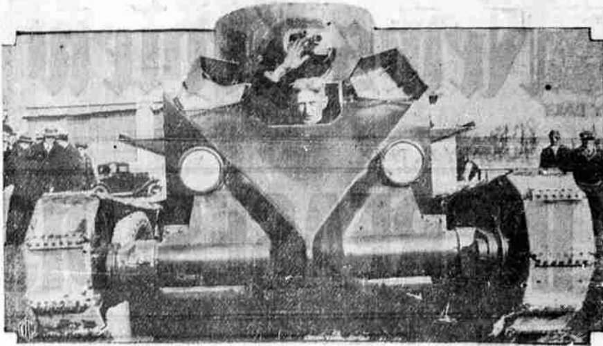
J. Walter Christie, famous automotive engineer, waving from the port of his new super-speed tank which was demonstrated to military authorities at Linden, N. J. It is not only the fastest tank in the world, but also the best equipped for fighting purposes, possessing 5/8-inch armor and carrying one-pounder cannon and 30 calibre machine guns with 2100 rounds of ammunition.
