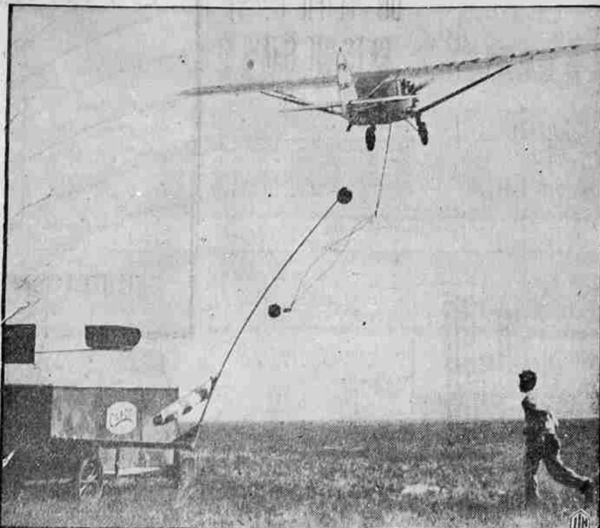
Roger Wolfe Kahn, son of the noted international banker, Otto H. Kahn, was at the controls of this plane during tests by the postoffice department to decide the feasibility of installing the Cabot aerial pickup device on regular airmail routes to facilitate faster delivery of mail. Photo shows a successful pickup. Note the dangling mailbag after the contact.
