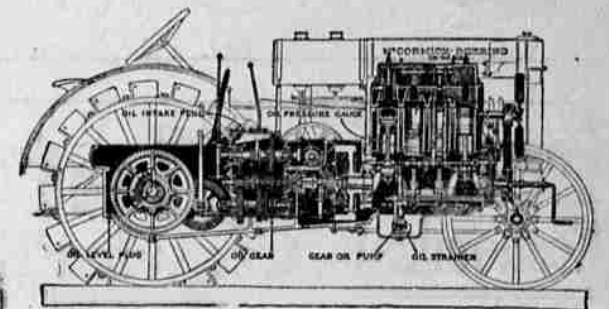
Cross section of the McCormick-Deering tractor.
