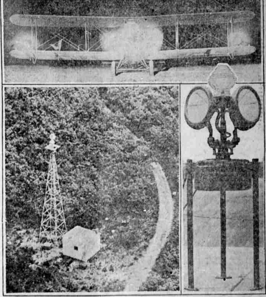
One hundred and fifty beacons of varying degrees of brilliancy, which mark the route of the new night air mail service between Chicago and New York, represent months of toil on the part of engineers, who had to blaze a trail of light in the sky under all sorts of conditions. A plane is seen preparing to leave Chicago. At left is a beacon in the wilderness, where there isn't a place to land in miles. At right is seen the type of beacon used: four powerful lights mounted on turn table base.
