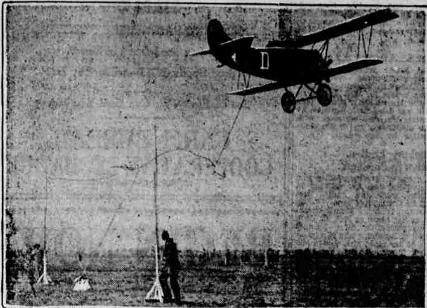
NON-STOP AIR MAIL COLLECTION —German mail planes are now experimenting with this ingenious method of picking up mailbags without stopping. The bags are attached to ropes between two poles and the pilot "drags his anchor" to snatch them up.
