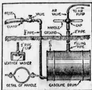
Pressure From Air Pump Is Used for Raising Gasoline From This Cheaply-Made Underground Storage Tank.
