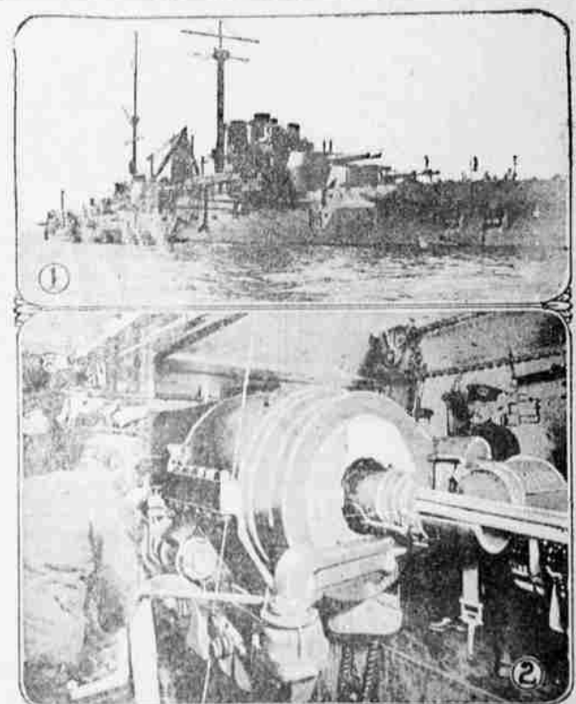
1. TYPE OF NEW FRENCH BATTLESHIP; 2. LOADING BIG GUN IN TURRET OF FRENCH BATTLESHIP.
