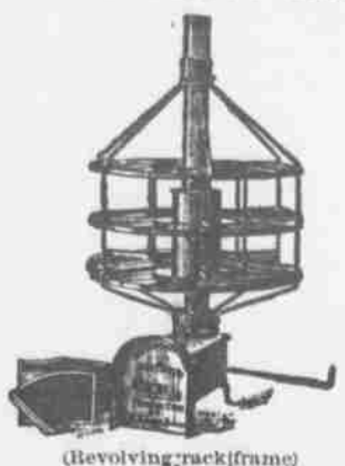
(Revolving rack frame)
